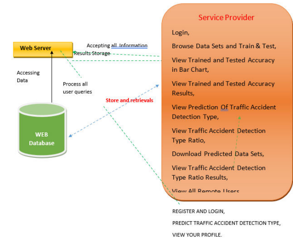
Fig 5.1: System Architecture
